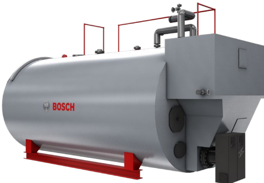
Figure 3: Hybrid boilers with electrical heater rods generate up to 5 MW of CO 2 -neutral process heat with regenerative energy usage. The burner of the Bosch boiler reliably covers additional demand.
